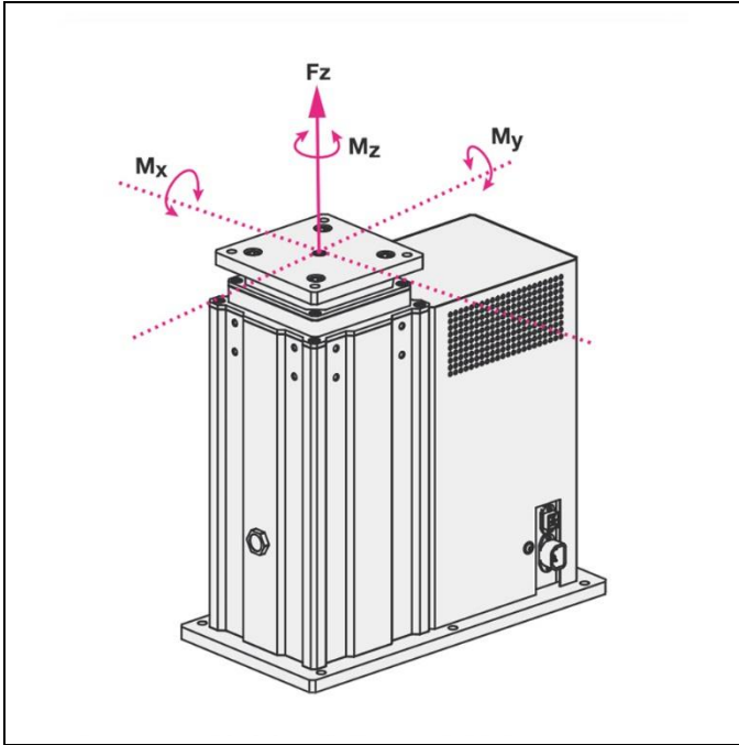
Figure 8: Side loads
