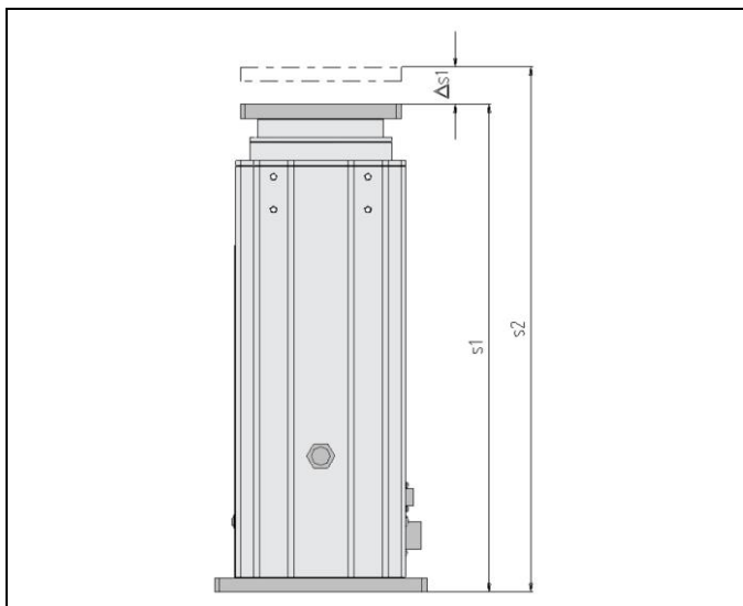
Figure 6: Determination of the axial thread backlash
